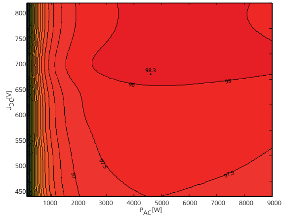
3D efficiency diagram for Powador 9.0 TL3
