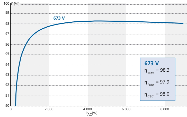
Efficiency characteristic curve for Powador 9.0 TL3
